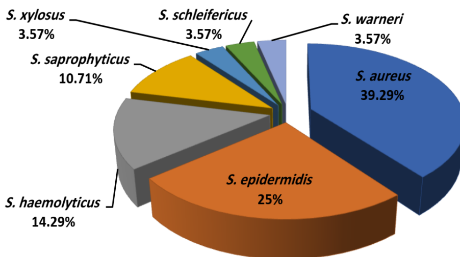
Fig. 1. The frequency of bacterial species isolated.
